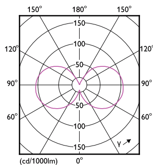
LEDbulb_A60_E27_806lm_FR
