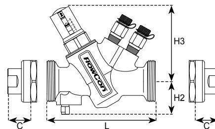
FlowCon ABV with E-JUST cartridge
