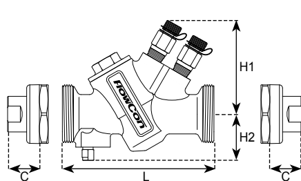
FlowCon ABV with composite cartridge
